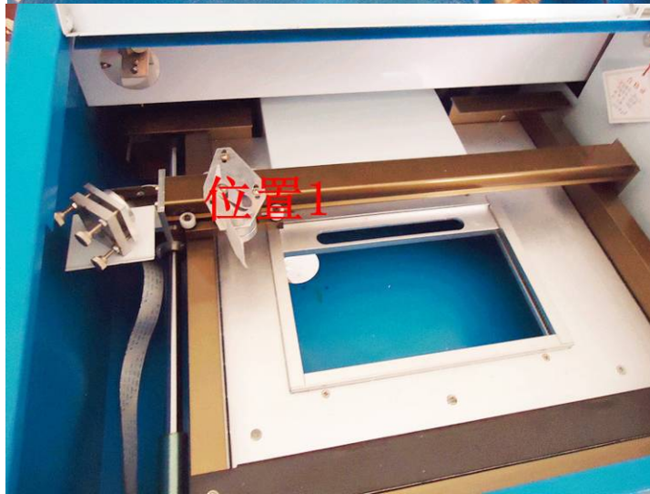
Figure 9 Step 8,move the laser head slowly to the side far from 2# mirror ,push Test switch to get a laser
